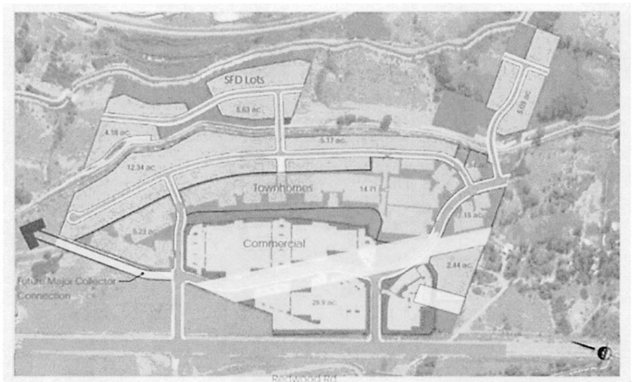
FIGURE 5 CONCEPTUAL SITE PLAN
