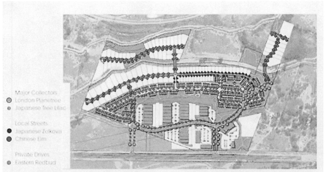
FIGURE 9 STREET TREE PLAN
