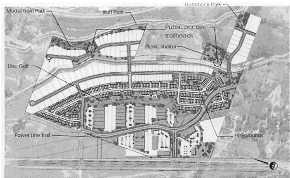
FIGURE 6 OPEN SPACE PLAN
